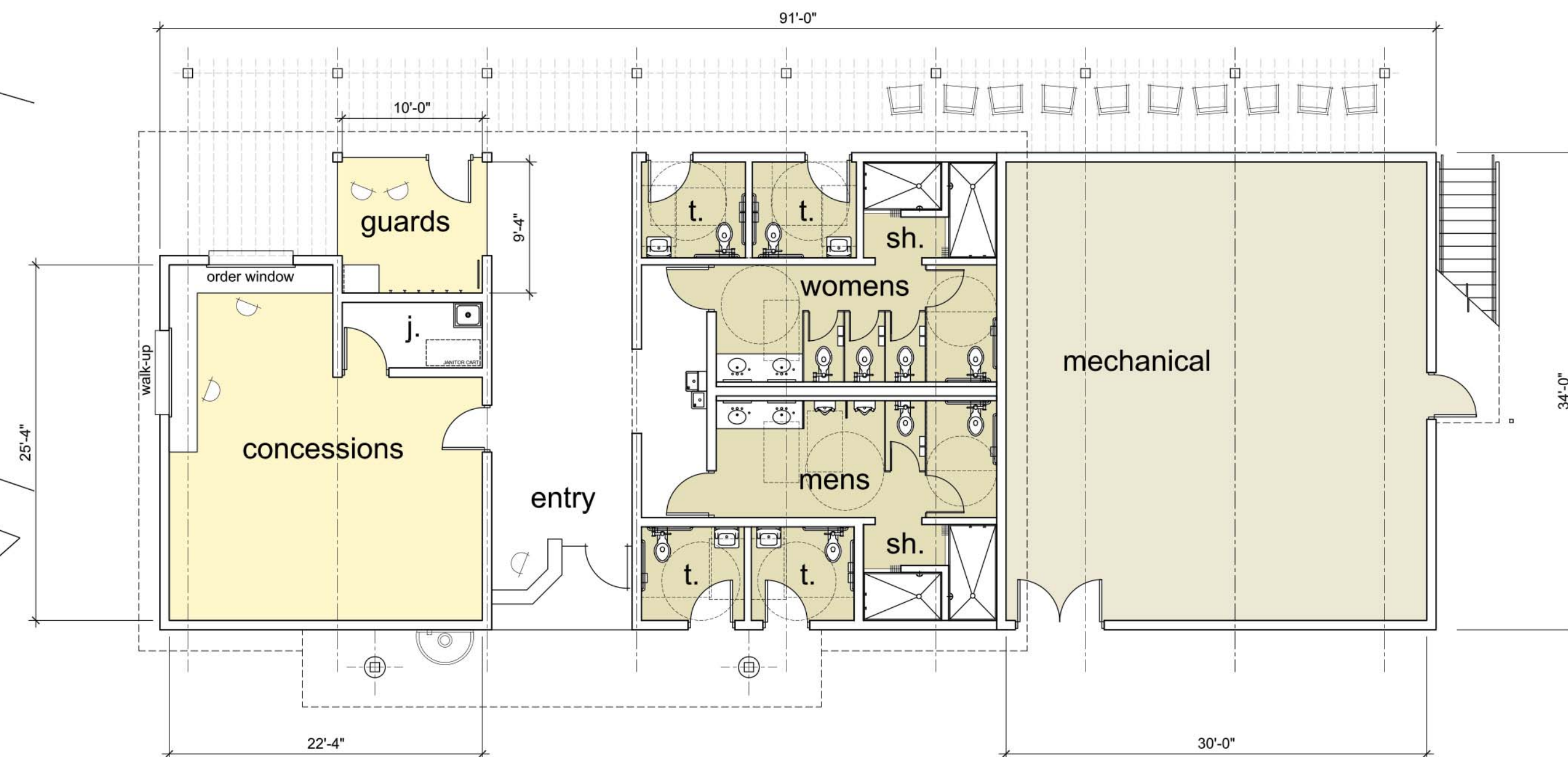
FLOOR PLAN 1/8" = 1'-0"
